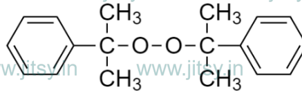
Di-Cumyl Peroxide
